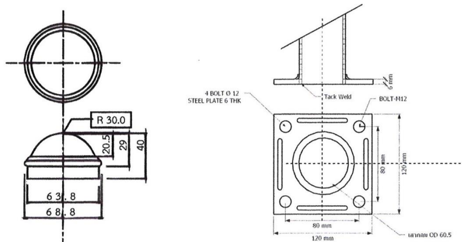
5 DETAIL ACCESSORIES
